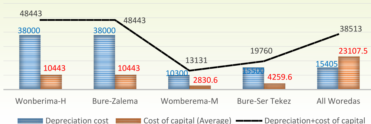
Figure 4: Depreciation and cost of capital for maize sheller in different areas (Birr)
