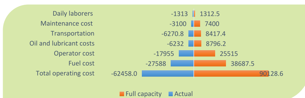
Figure 3: Actual and potential operating costs- multi-crop thresher
