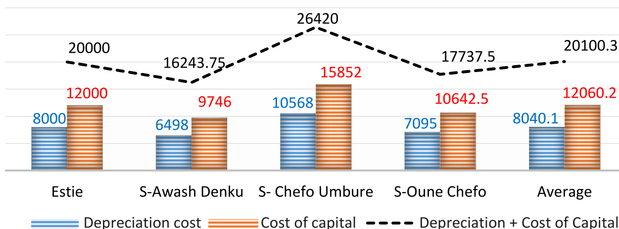
Figure 5: Depreciation and cost of capital for multi-crop thresher in different areas (Birr)
