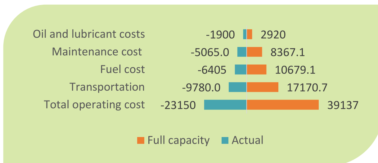
Figure 1: Actual and potential operating costs-Bako model
